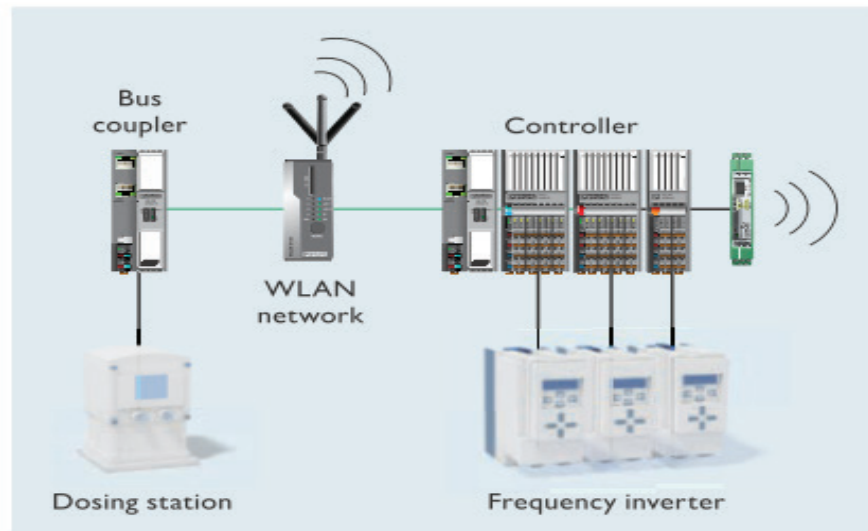
Operational building with dosing station and drive technology
